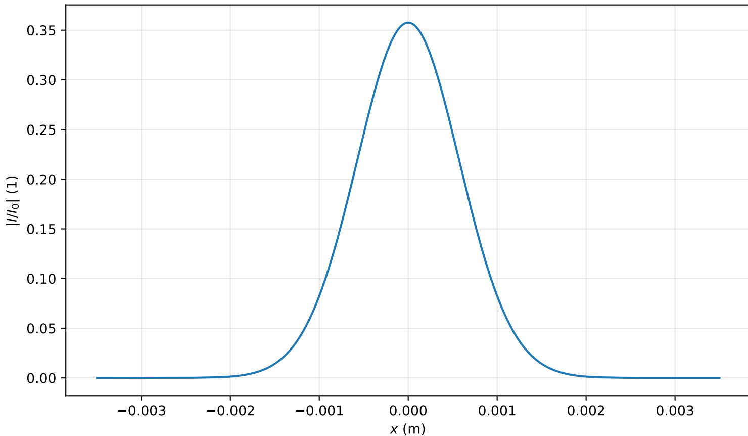
Intensity profile I(x, y = 0, z = 2.866m)/I_0 , P_{in}=0.1P_{cr} , artificial time
